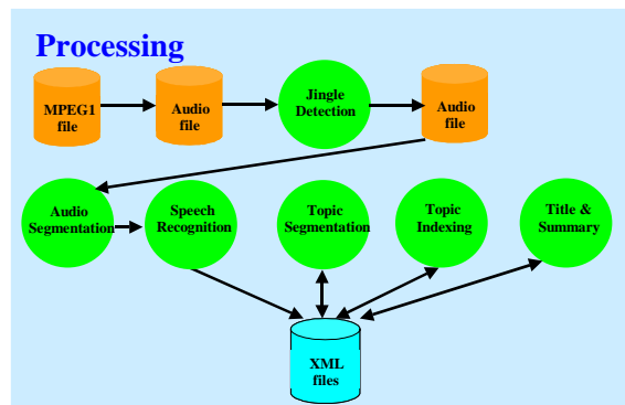
Figure 2 - Functional diagram of the Processing block.
