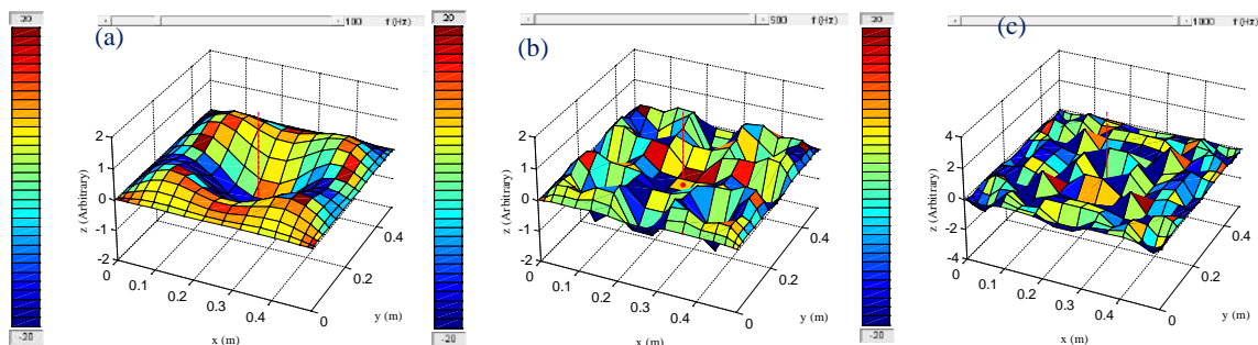
Figure 4: 3D deformation of fibreglass composite simply supported plate at a) 100 Hz, b) 500 Hz, and c) 1 kHz.
