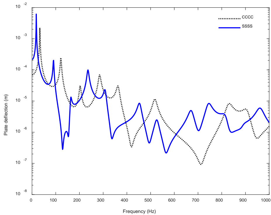
Figure 3: Deflection of simply supported and clamped fibreglass plate at x = 0.15 m and y = 0.15 m
