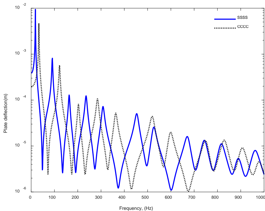
Figure 2: Deflection of simply supported and clamped fibreglass plate at x = 0.25 m and y = 0.25 m
