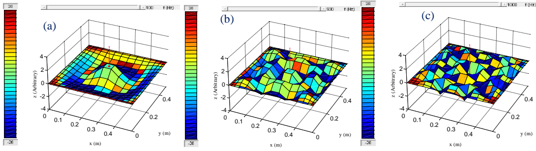
Figure 5: 3D deformation of fibreglass composite clamped plate at a) 100 Hz, b) 500 Hz, and c) 1 kHz respectively.
