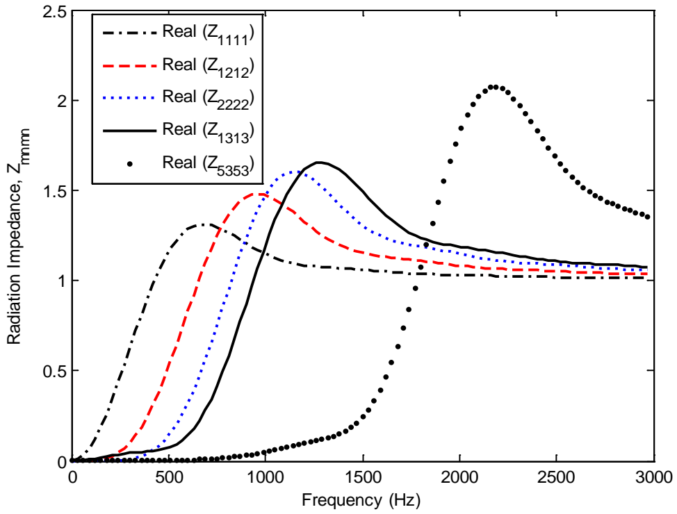
Figure 6: Radiation impedance matrix, direct terms.
