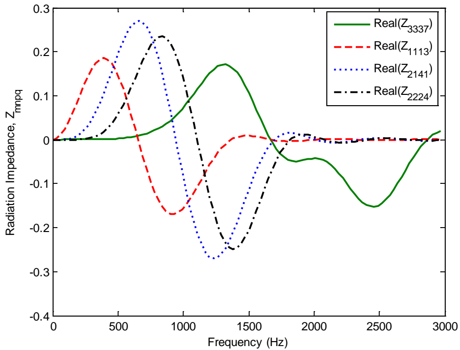
Figure 7: Cross coupling terms of the real part of the radiation impedance matrix
